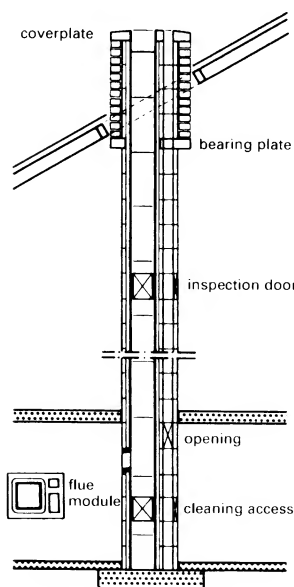
15 Modular flue installation
